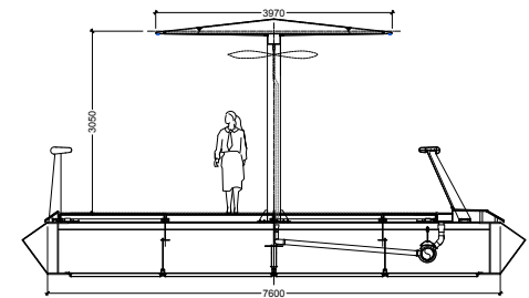
Deck Typical Section
